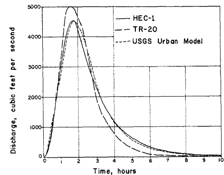
FIGURE 2. Unit hydrographs for Deep Fork Creek at Eastern Avenue
