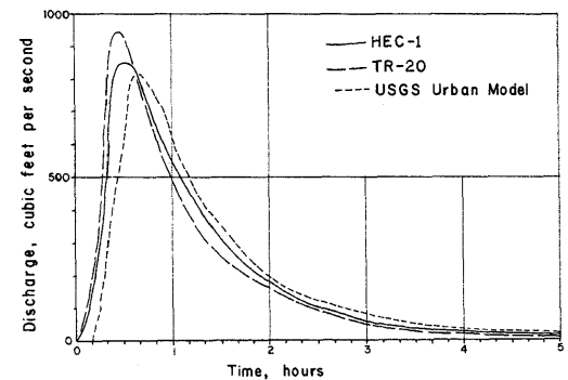
FIGURE 3. Unit hydrographs for Bluff Creek at Northwest Highway
