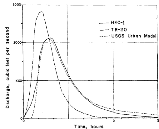
FIGURE 1. Unit hydrographs for Deep Fork Creek at Portland Avenue
